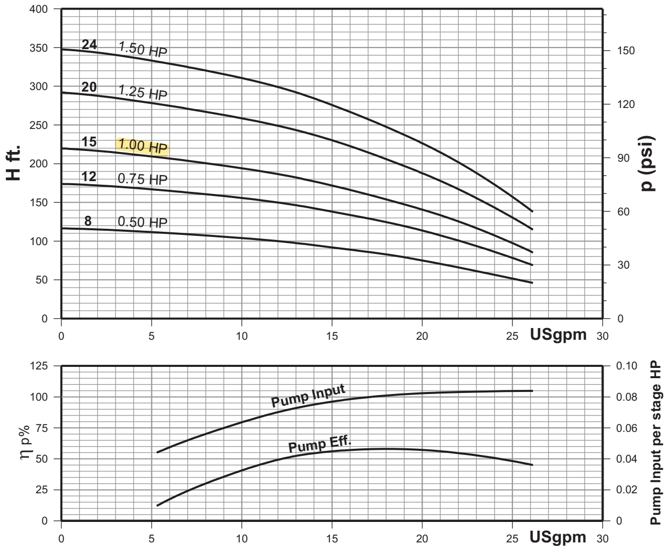
Performance Curve
